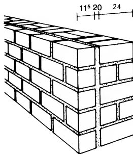
③ Double leaf with brick facing
